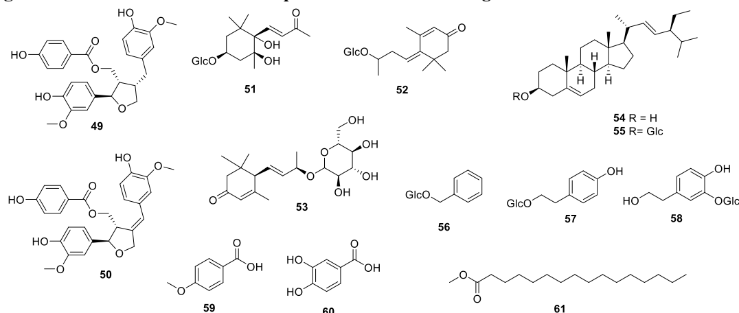
Figure 4. Chemical structure of compounds 49-61 from A. rugosa
