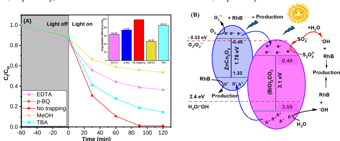
Fig.4 (A) Effects of radical scavengers on RhB degradation; (B) Schematic diagram of the mechanism of RhB decomposition of PS-activated BiC@ZC
