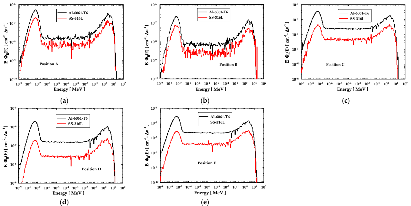
Figure 3. Comparisons of neutron spectra at positions A, B, C, D, and E in the NC-9000 reactor with Al-6061-T6 and SS-316L tubes: (a) Lateral near-core, (b) lateral elevated, (c) top experimental zone, (d) upper instructional area, and (e) reactor top center above the ^{239}\text{PuBe} source.
