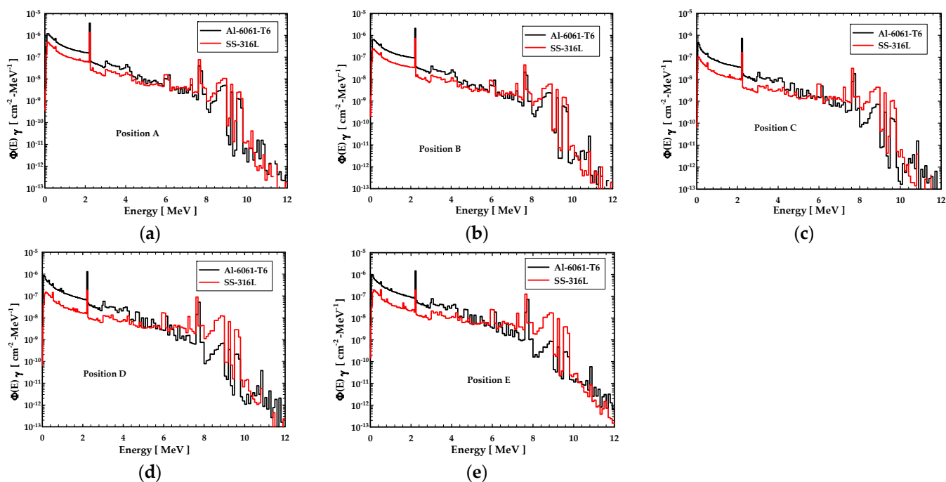
Figure 4. Comparison of gamma-ray spectra at the different detector positions in the NC-9000 reactor, with Al-6061-T6 and SS-316L tubes: (a) Lateral near-core, (b) lateral elevated, (c) top experimental zone, (d) upper instructional area, and (e) reactor top center above the ^{239}\text{PuBe} source.
