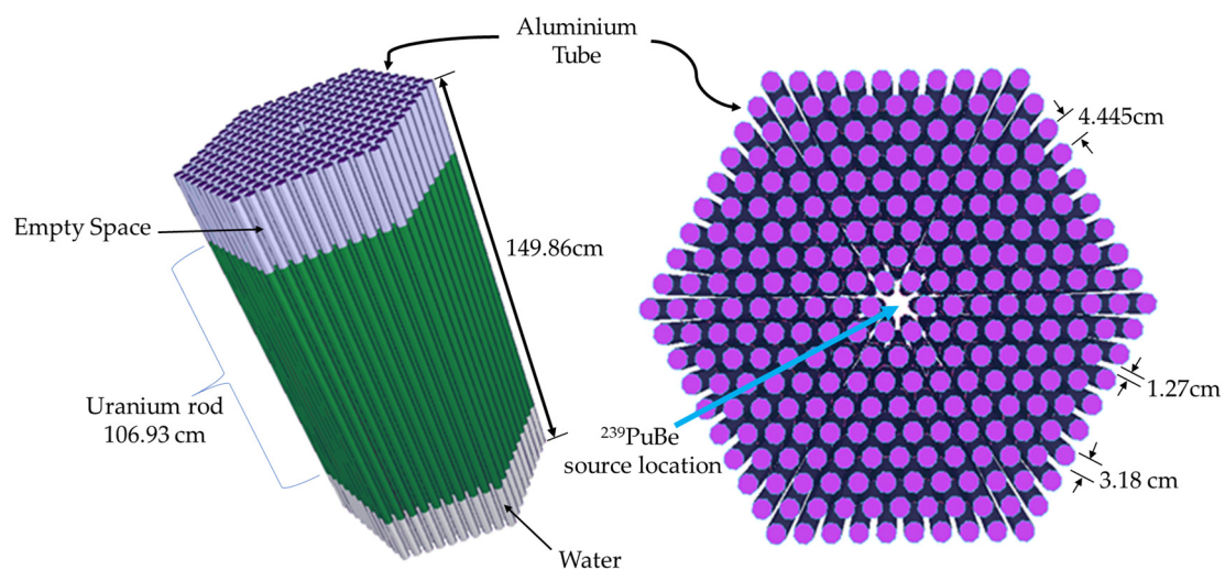
Figure 1. A three-dimensional view of the NC-9000 subcritical reactor showing the hexagonal array of 270 fuel tubes. The core has a maximum diameter of approximately 88.9 cm. The central ^{239}\text{PuBe} neutron source is located at the center of the core. Each fuel tube contains natural uranium slugs surrounded by light water, which serves as both a moderator and a reflector.
