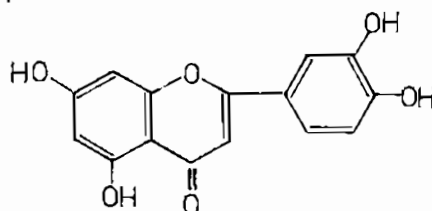
Luteolin
