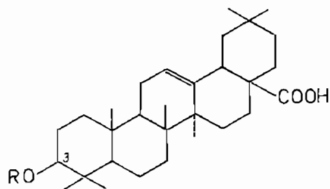
Acid oleanolic C_{30}H_{48}O_3 R = H
