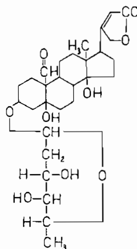
Corchorosid
