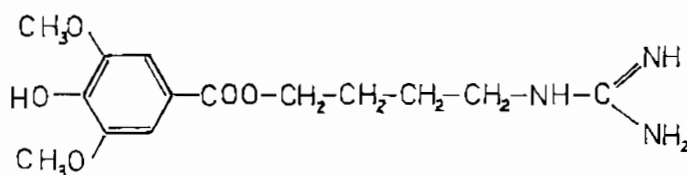
Leonurin
