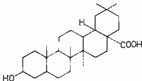
Acid oleanolic
