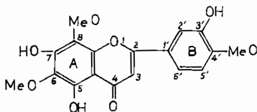
5, 7, 3' - Trihydroxy -6,8,4'- trimethoxy flavon
