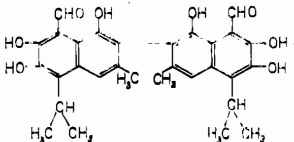
Gossypol
