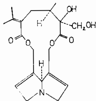
Mucronatin C_{18}H_{25}O_8N
