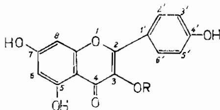
Quercetin
