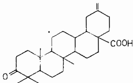
3 - Oxo-20 (30) urcen (28) ovic acid
