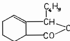
Cnidium lacton
