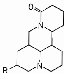
Matrin C_{15}H_{24}N_2O
