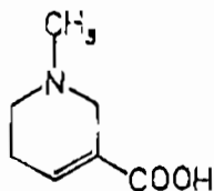
Arecaidin C_7H_{11}O_2N
