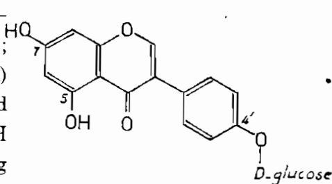
Sophoricosid
