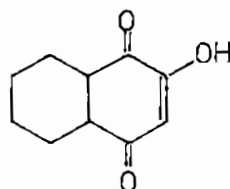
Lawson (hydroxyl 2-naphthoquinon 1-4)
