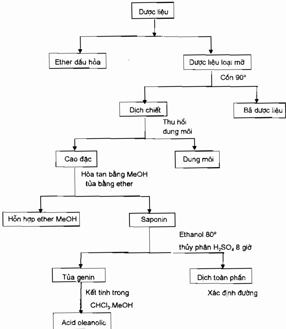
Acid oleanolic
