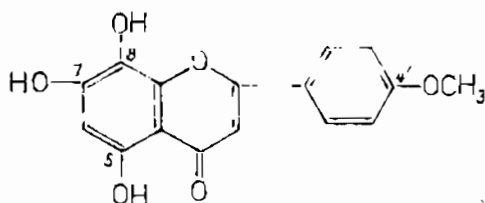
Chất (II) 5,7,8 - trihydroxy - 4' - methoxyflavon C_{16}H_{12}O_6
