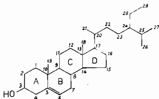
\beta -Sitosterol
