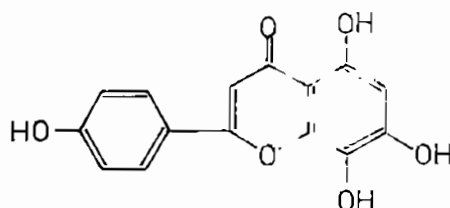
5, 7, 8, 4' – Tetrahydroxyflavon
